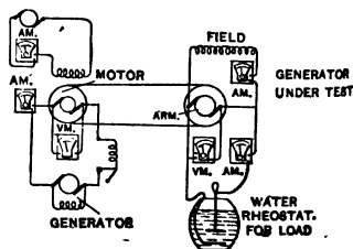
FIG. 5. Connections for efficiency test of a generator. Driven by an electric motor.
