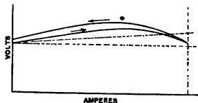
FIG. 36. Characteristic of Over-compounded Compound-wound Dynamo.
