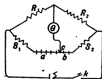
FIG. 9. Cary-Foster Bridge.
