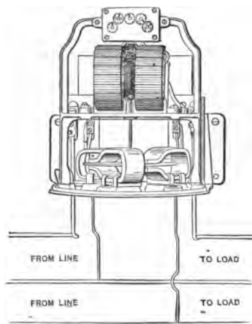
FIG. 7. Balanced Three-phase Secondary Meter.
