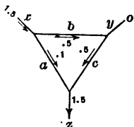
FIG. 62. Path and Value of Current in Delta-connected Armature.
