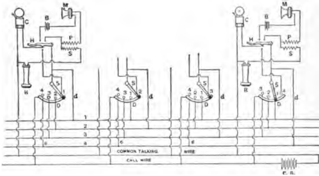
FIG. 53. Common Signaling Battery System; Individual Talking Batteries.
