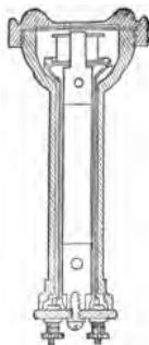
FIG. 8. Double Pole Receiver.
