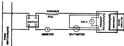
FIG. 64. Impedance Test with Wattmeter.
