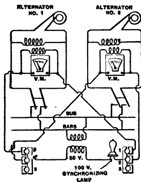
FIG. 64. Synchronizer Connections.
