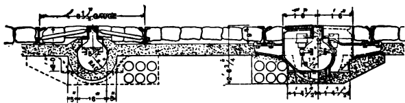
FIG. 94. Section of Conduit, Metropolitan Street Railway, New York. — Standard Work, 1897-98.
