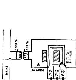
FIG. 20. Westinghouse Economy Coil. For A.C. arc lamps.
