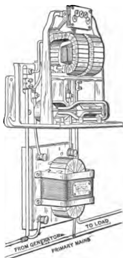
FIG. 4. Primary Meter.
