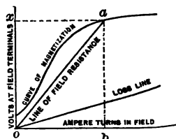
FIG. 35. Internal Characteristic of Shunt Dynamo.
