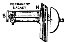
FIG. 24. Polarized Bell with long core for Ringer of Bridging-Bell.
