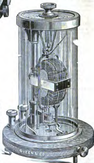
FIG. 30. Siemen's Electro-Dynamometer.
