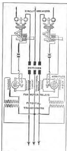
FIG. 22. The Circuits of a Reverse Current Circuit Breaker Set Showing How a Direct Current Motor is Used with Alternating Currents to Distinguish between Power Passing in One Direction and Power Passing in the Other Direction in the Line.
