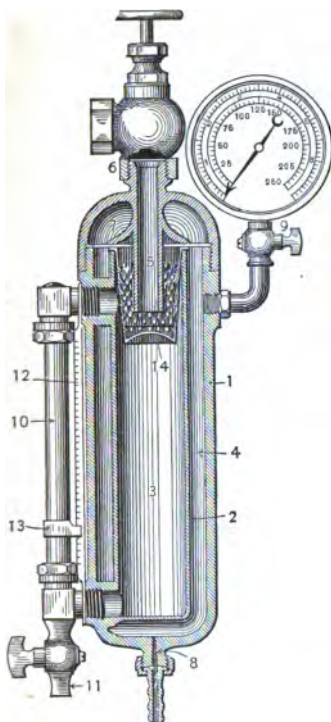
FIG. 10. Carpenter's New Evaporating Calorimeter. (Schaeffer & Budenberg.)
