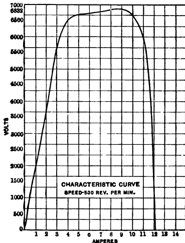
FIG. 30. Characteristic curve of Brush 125-Light Arc Dynamo without Regulator.
