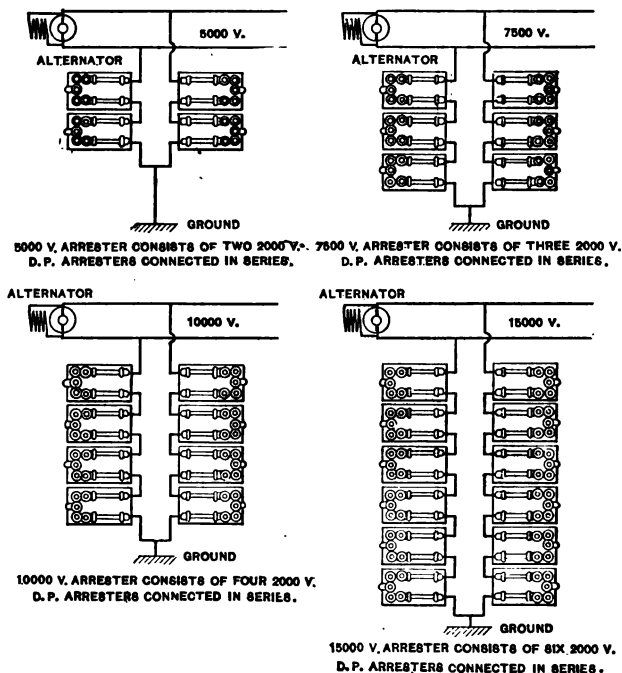
FIG. 21. Connections of Wirt or G. E. Alternating Current Short Gap Lightning Arresters, 5000 to 10,500 volts.
