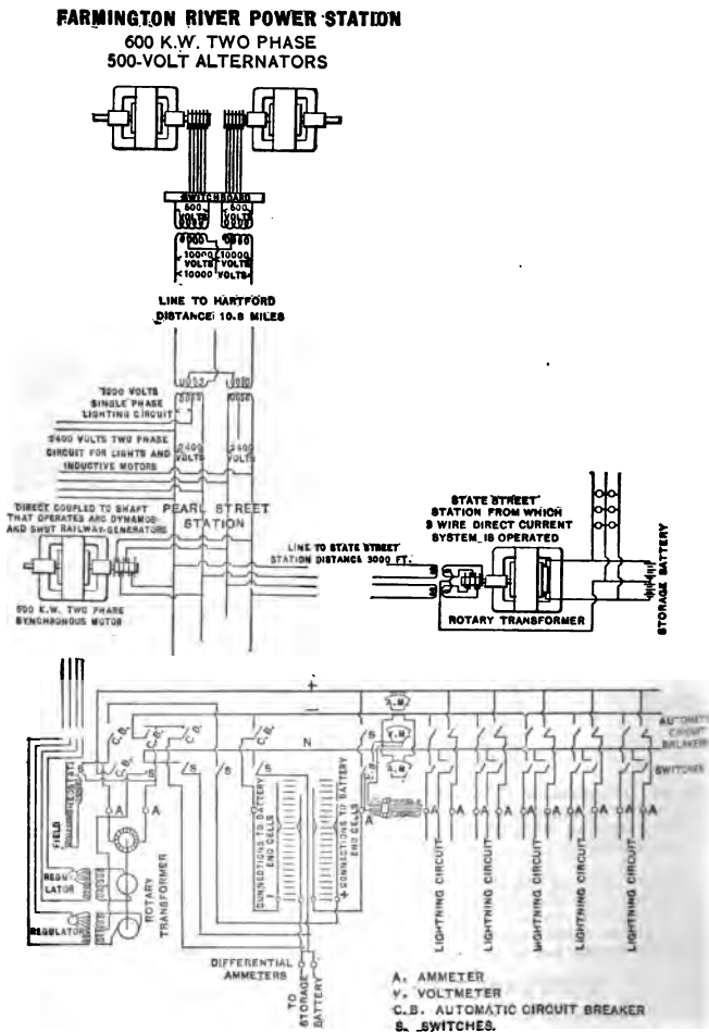
Figs. 31 and 32. Connections of Machines and Circuits of Hartford Electric Light Company, showing Special Connection of the Storage Battery to Rotary Converters.
