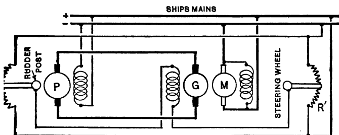
FIG. 6. Diagram of Steering-Gear.
