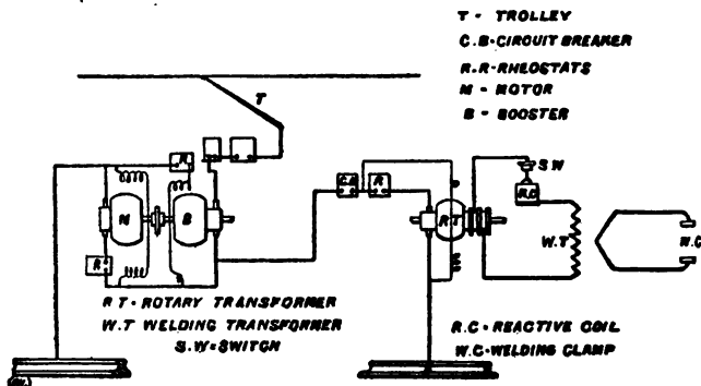
DIAGRAM OF CONNECTIONS OF RAIL WELDER
