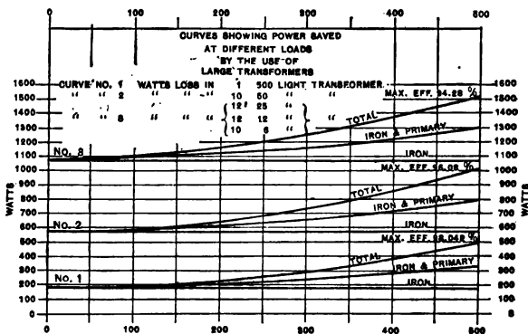
FIG. 13. Relative Efficiency of Large and Small Transformers.
