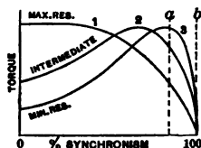
FIG. 72. Torque curves for Polyphase Induction Motor.
