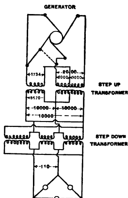
FIG. 58. Changing Quarter-phase to Three-phase, and back to Quarter-phase. All Transformers Interchangeable.
