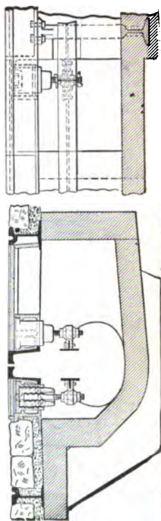
FIG. 91. Plan and Section of Conduit, showing G Conductor Support, Metropolitan Railroad, Washington, 1895.
