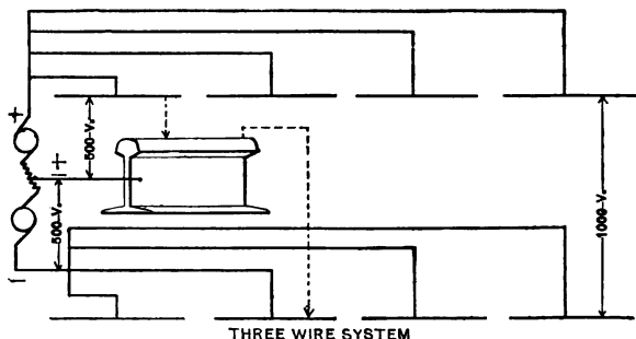
FIG. 68. Three-Wire System.
