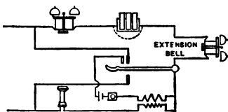
FIG. 17. Diagram showing proper Connections of Extension Bell.
