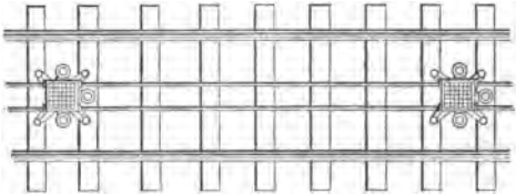
FIG. 103. Track Equipped for Insulating Return Circuit.
