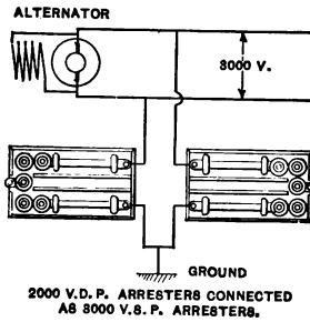
FIG. 22. G. E. Alternating Current Lightning Arresters.
