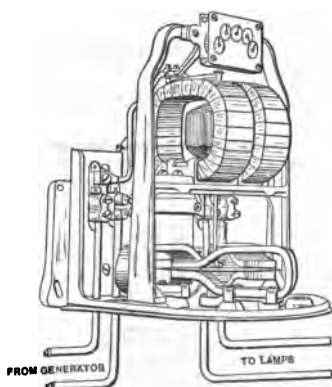
FIG. 1. Two-wire Meter. (Small Capacity.)
