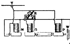
FIG. 67. Leonard's System of Electric Propulsion.
