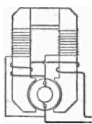
COMPOUND WOUND DYNAMO SHORT SHUNT FIG. 22.
