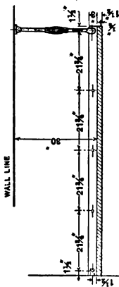
FIG. 3. Showing Method of Bracing Switchboard Panel to Wall.
