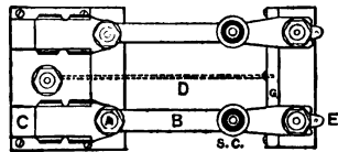
FIG. 22. Plan of Combination Protector.
