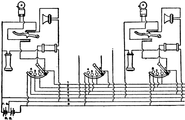
FIG. 54. System having Common Talking and Signaling Battery.
