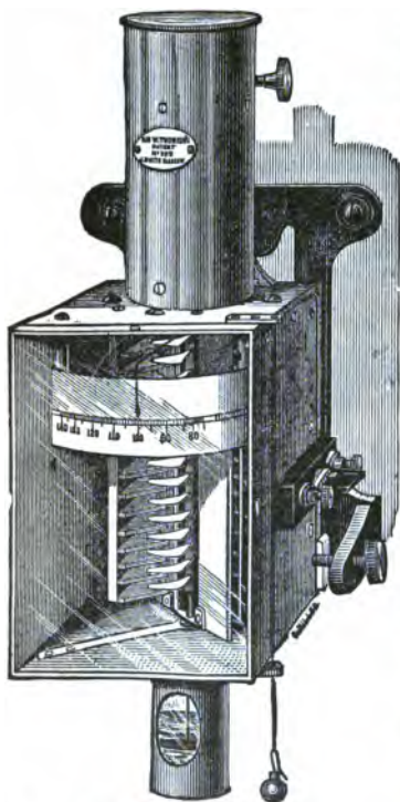
FIG. 29. Another Form of Lord Kelvin's Electrostatic Voltmeter.
