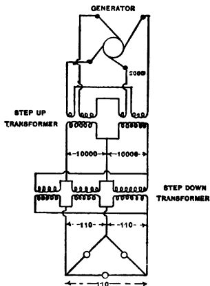
FIG. 56. Changing Quarter-phase to Three-phase, Non-interchangeable Step-up Transformers.
