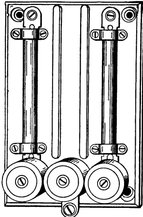
FIG. 22. G. E. Alternating Current Lightning Arresters.
