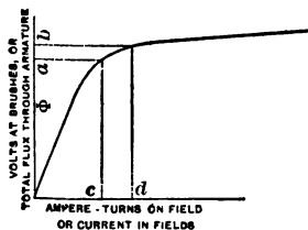
FIG. 28. Magnetization Curve.
