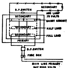
FIG. 27. Diagram of Connections.
