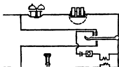
FIG. 16. Diagram of Connections of Series Magneto Bell and Telephone Set.
