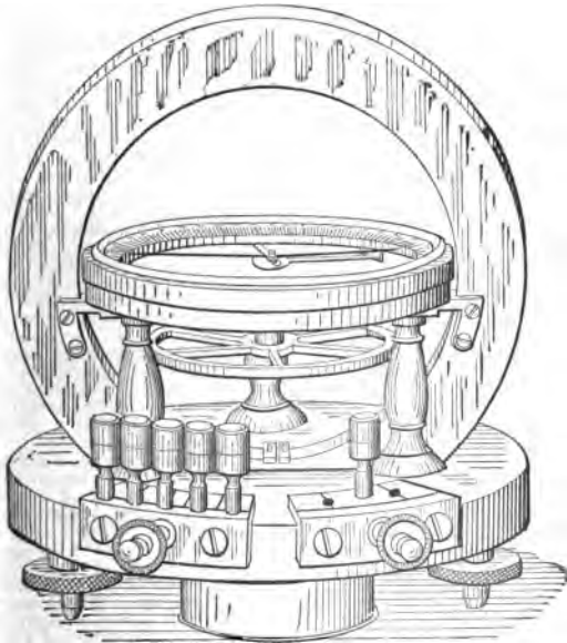
FIG. 11. Tangent Galvanometers.
