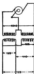
FIG. 54. Monocyclic Connections.
