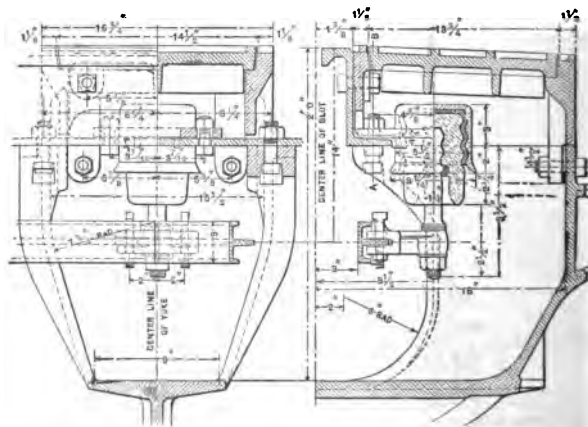
FIG. 97. Section and Elevation of Insulator, Metropolitan Street Railway, New York. — Standard Work, 1897-98.
