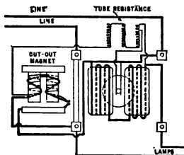
FIG. 13. Arc Circuit Meter.
