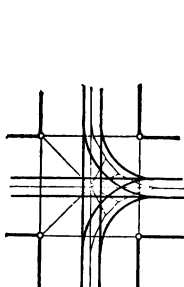
FIG. 25. Single-Track Crossing, Cross Suspension.
