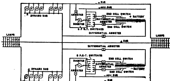
FIG. 24. Circuits of Storage Batteries in Connection with Three-Wire System, Philadelphia Edison Station.
