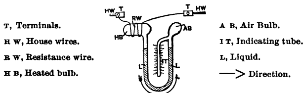
FIG. 47. Wright Discount Meter.
