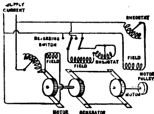
FIG. 66. Leonard's System of Motor Control.
