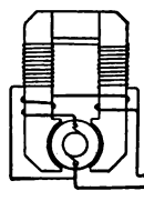
COMPOUND WOUND DYNAMO LONG SHUNT FIG. 23.
