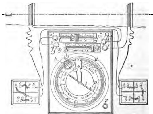
FIG. 6. Connections of Schmidt Chronograph.
