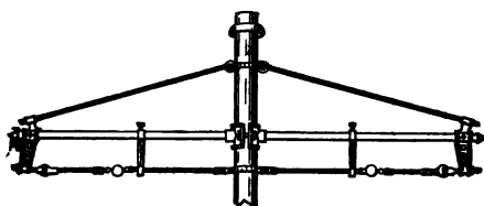
FIG. 16. Double Suspension. For Iron Poles.
