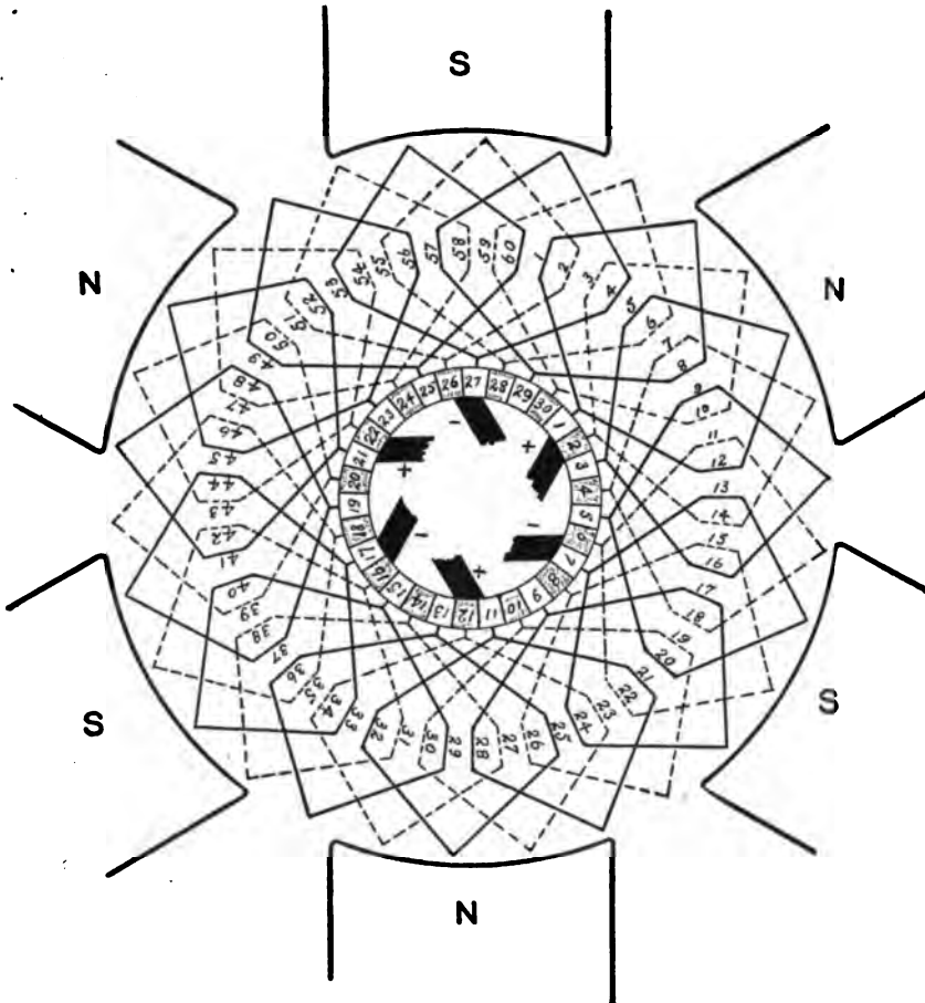
Six-pole drum duplex lap winding, doubly reëntrant. Z = 60 , front pitch = -11 , back pitch = +7 , commutator pitch = -2 , number of paths = 12 .
