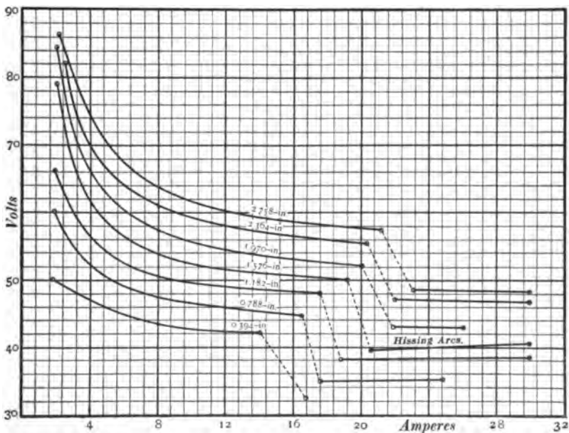
Fig. 183. Volt-ampere characteristics of an open direct-current arc between solid carbons one half inch in diameter.
