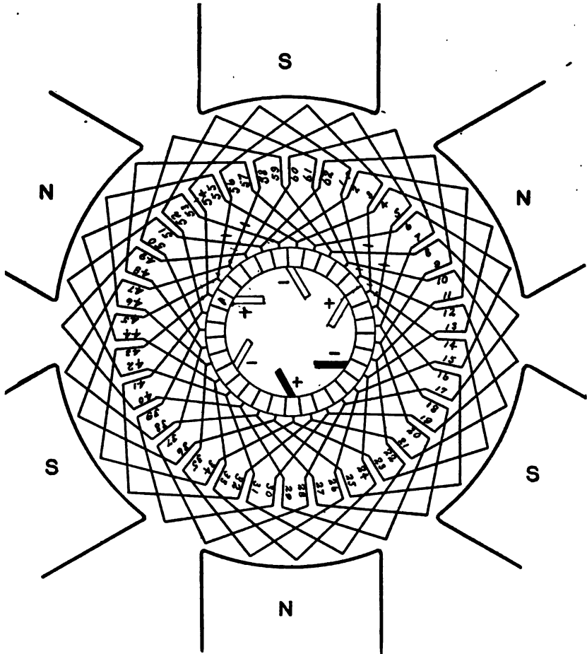
Six-pole drum simplex wave winding. Z = 62 , front pitch = +11 , back pitch = +9 , average pitch 10, commutator pitch +10 , number of paths = 2 .
