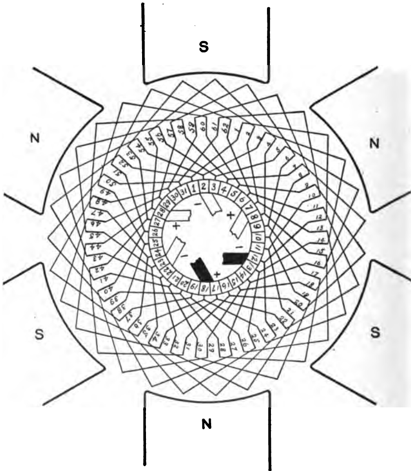
Six-pole drum duplex wave winding, singly reentrant. Z = 62 , front pitch = +11 , back pitch = +11 , average pitch = 11 , commutator pitch = +11 , number of paths = 4 .
