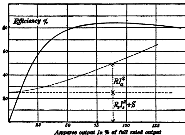
Fig. 95. Efficiency and loss curves of a shunt generator.
