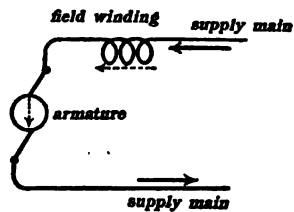
Fig. 78. Series Motor.
