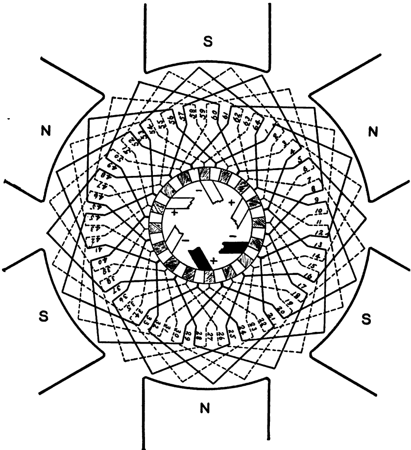
Six-pole drum duplex wave winding, doubly reëntrant. Z = 64 , front pitch = +9 , back pitch = +11 , average pitch 10, commutator pitch 10, number of paths = 4 .
