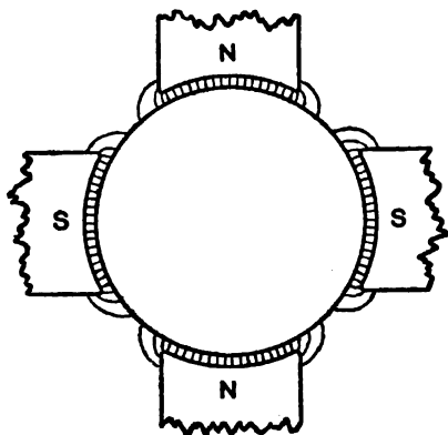
Fig. 97. Undistorted field of a dynamo when armature current is small.
