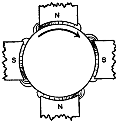
Fig. 99. Same as Fig. 98, but showing motor distortion for same direction of running.
