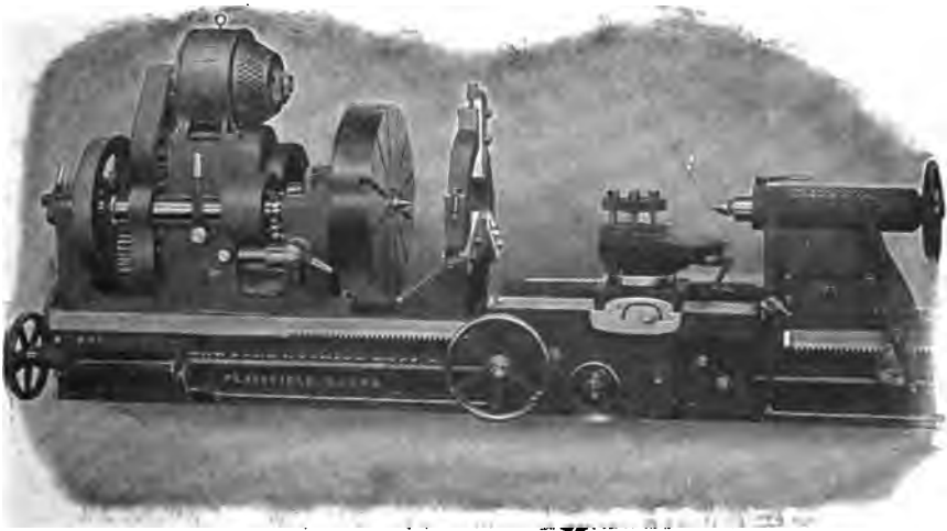
Fig. 59. Westinghouse Variable Speed Motor Driving a 48-inch Lathe.
