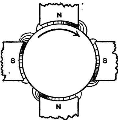
Fig. 98. Distorted field of a generator when its armature current is large.
