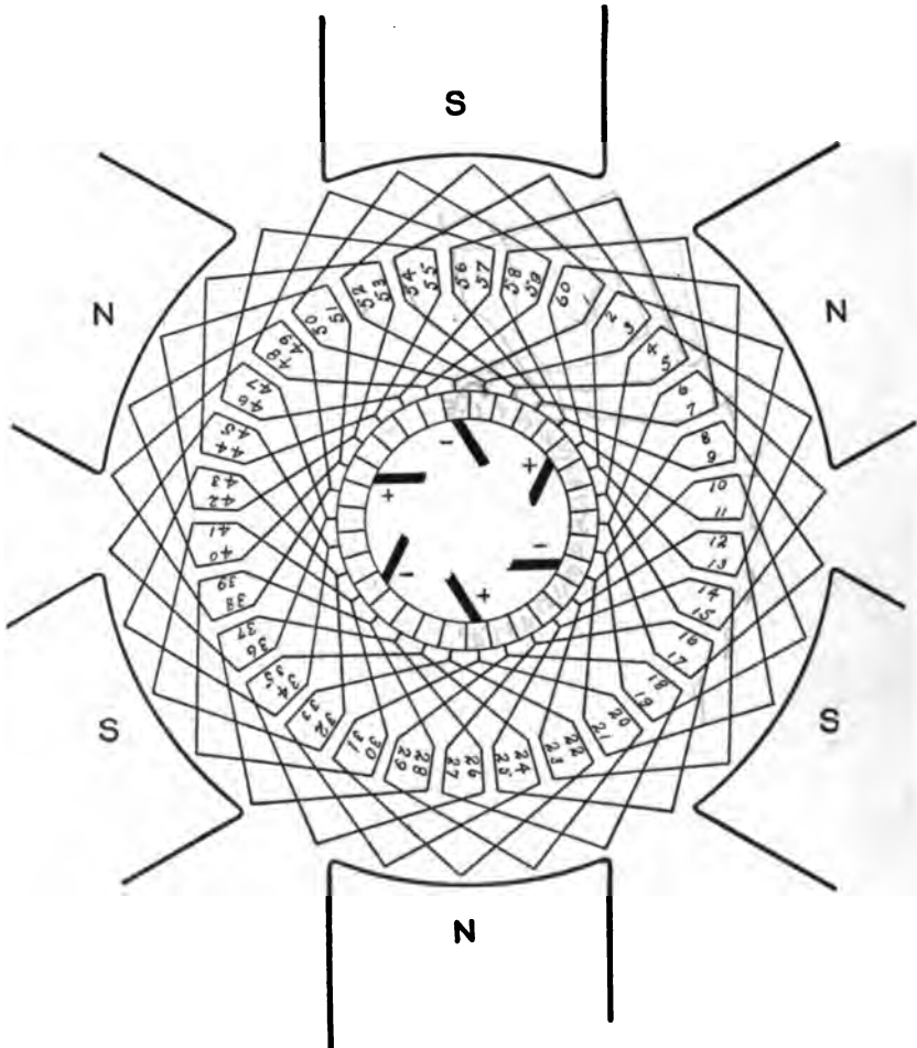
Six-pole drum simplex lap winding. Z=60 , front pitch = -11 , back pitch = +9 , commutator pitch = -1 , number of paths = 6 .
