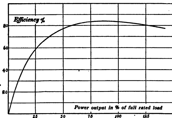
Fig. 96. Efficiency Curve of a Shunt Motor.
