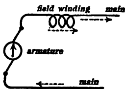
Fig. 77. Series Generator.
