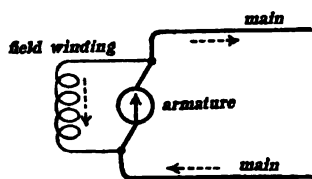
Fig. 75. Shunt Generator.
