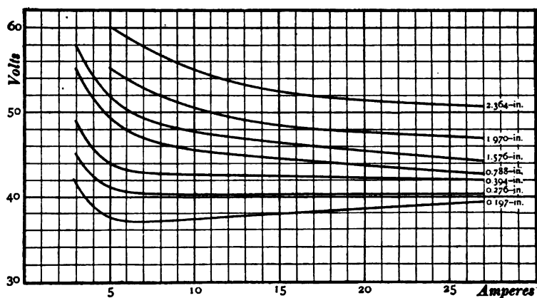
Fig. 182. Volt-ampere characteristics of an open direct-current arc between cored carbons one half inch in diameter.
