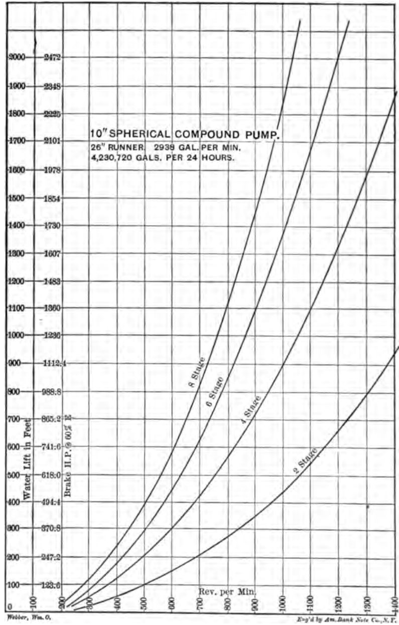
FIG. 285.—HORSE-POWER AND SPEED CURVES COMPOUND PUMP.
