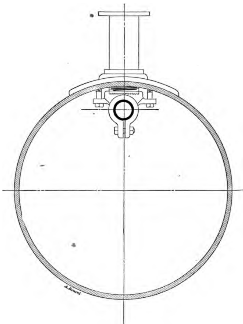
FIG. 227.—CROSS SECTION AT SAFETY VALVE.
