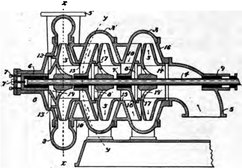
FIG. 269.—B. JACKSON'S SERIES HIGH-PRESSURE CENTRIFUGAL PUMP FOR HIGH HEADS.
