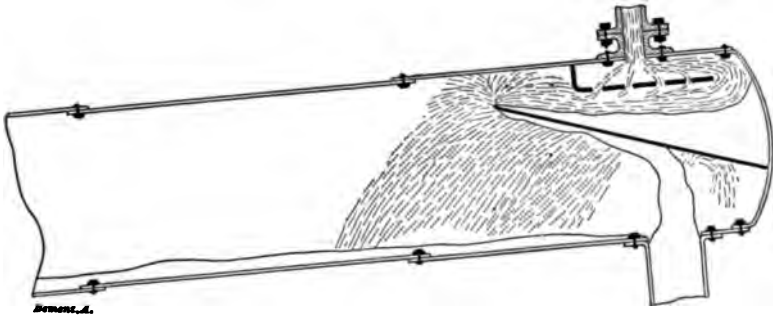
FIG. 100.—HEINE BAFFLE WITH LOW WATER LINE.
