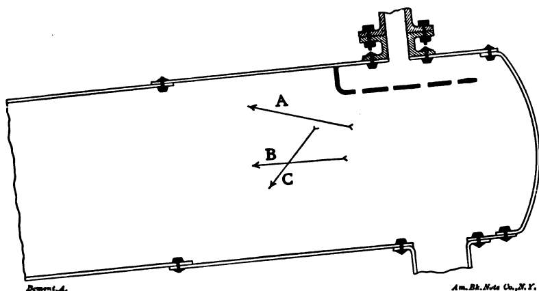
FIG. 107.—ANGLE OF DEFLECTION, DIFFERENT WATER BAFFLES.
