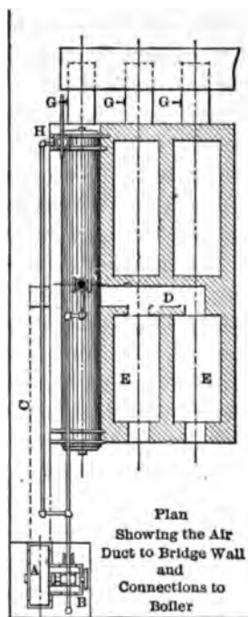
FIG. 238.—BALANCED DRAFT SYSTEM.
