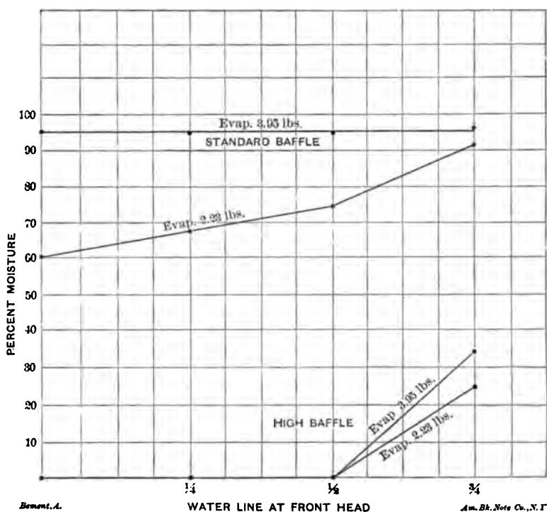
FIG. 97.—RESULTS OF TESTS OF BAFFLES.
