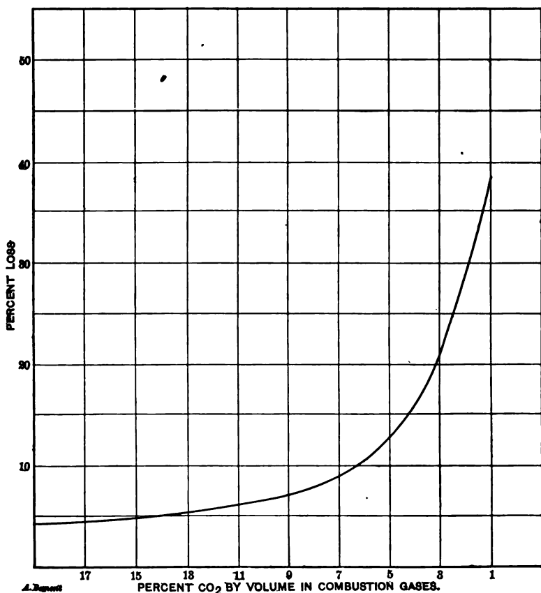
FIG. 235.—LOSS FROM BOILER A OVER B DUE TO DECREASING INITIAL TEMPERATURE, MEASURED ABOVE TEMPERATURE OF AIR.
