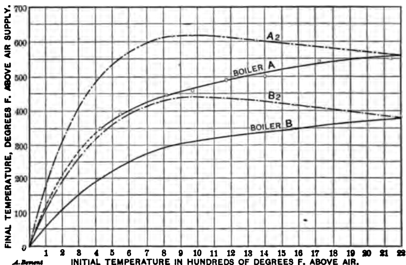
FIG. 236.—RELATION OF FINAL TO INITIAL TEMPERATURE.
