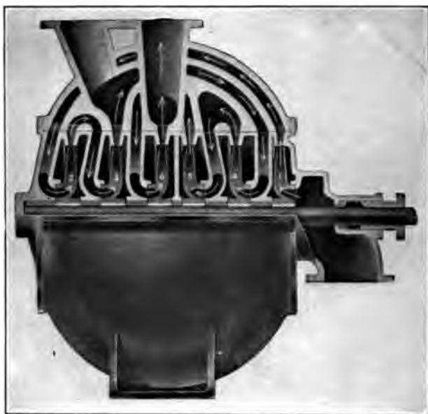
FIG. 275.—10-INCH SIX STAGE SPHERICAL PUMP.
