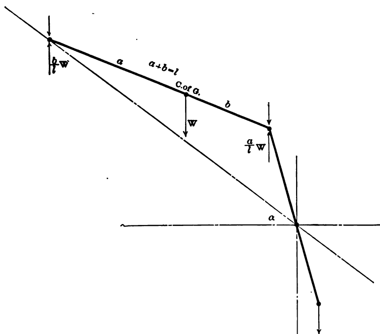
DIAGRAM OF CONNECTING ROD WEIGHT.
