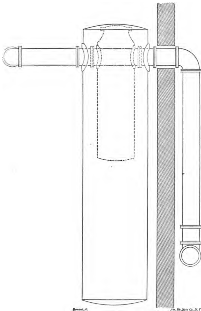
FIG. 109.—ELEVATION SHOWING DIFFERENT STEAM CONNECTIONS TO ENGINES K AND L.
