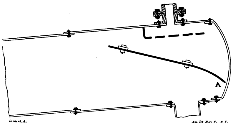
FIG. 115.—OLD STYLE BAFFLE. BOILER NO. 14.
