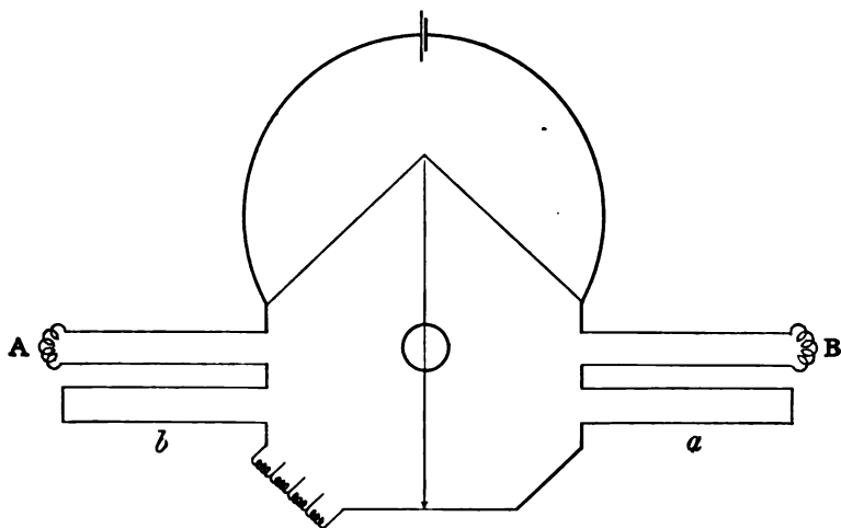
FIG. 206.—DIFFERENTIAL THERMOMETER CONNECTIONS.
