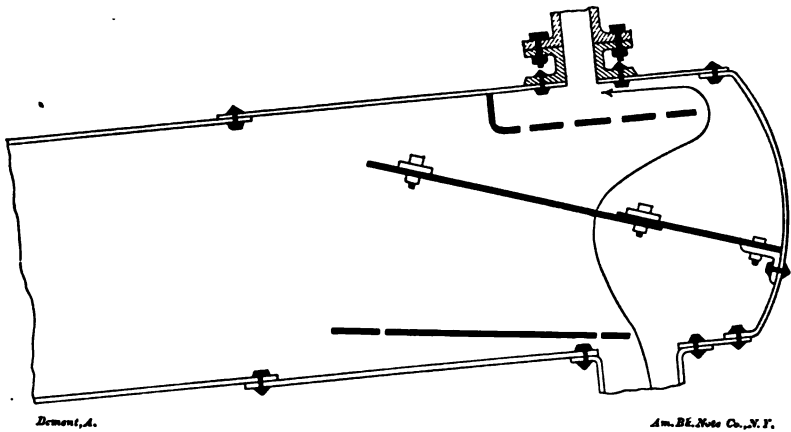
FIG. 112.—ELEVATION, PLATE COMPLETELY DETACHED.
