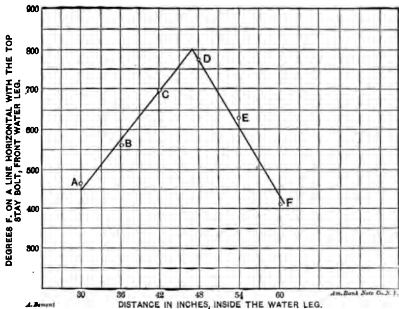
FIG. 232.—TEMPERATURE ACROSS GASES AT EXIT FROM TUBES.
