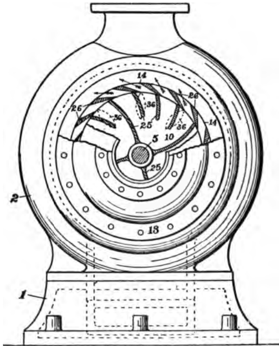
FIG. 272.—THE J. RICHARDS COMPOUND ROTARY PUMP.
