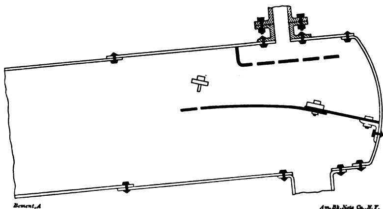
FIG. 111.—END OF BAFFLE PLATES DROPPING DOWN.
