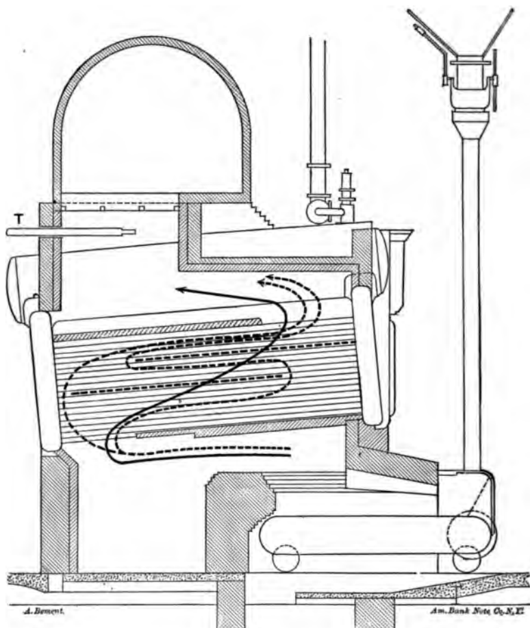
FIG. 230.—ELEVATION IN SECTION, SHOWING BOILERS A AND B.
