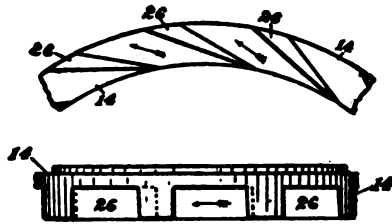
FIG. 271.—DETAILS OF THE J. RICHARDS COMPOUND ROTARY PUMP.
