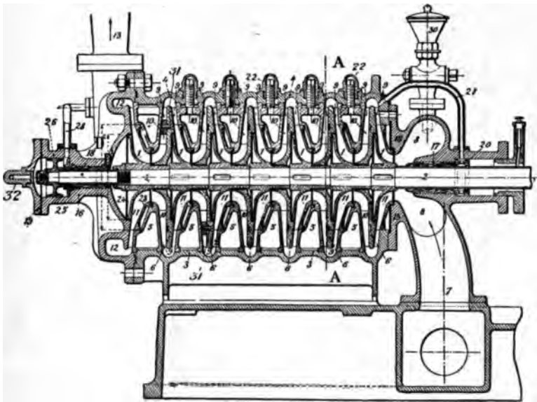
FIG. 266.—DETAIL OF THE A. C. E. RATEAU CENTRIFUGAL PUMP.
