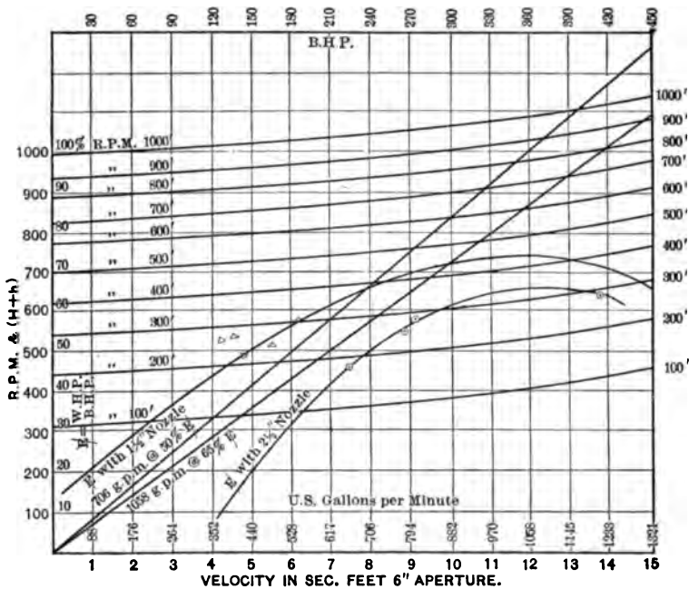
RATING SHEET & TESTS. 6" 6 STAGE SPHERICAL PUMP.
