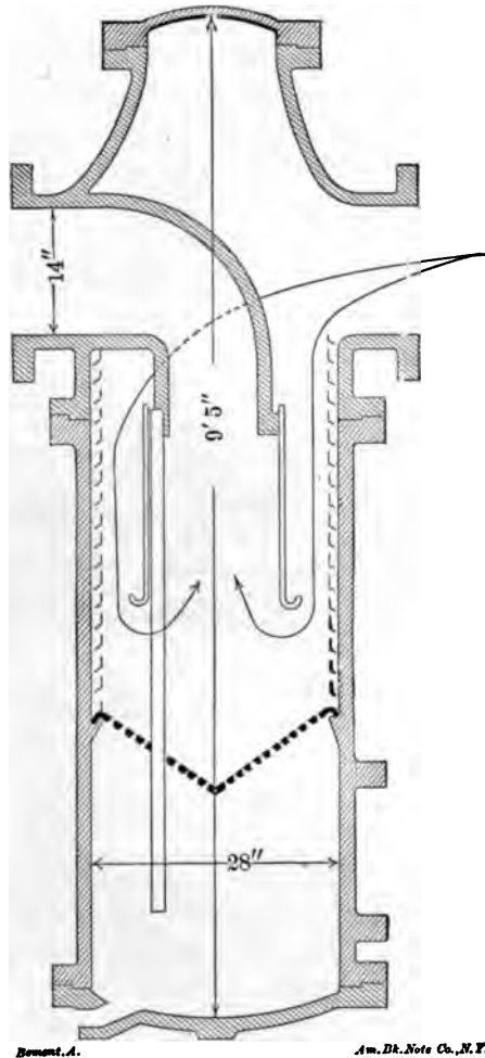
FIG. 96.—SMALL SEPARATOR, ENGINE K.
