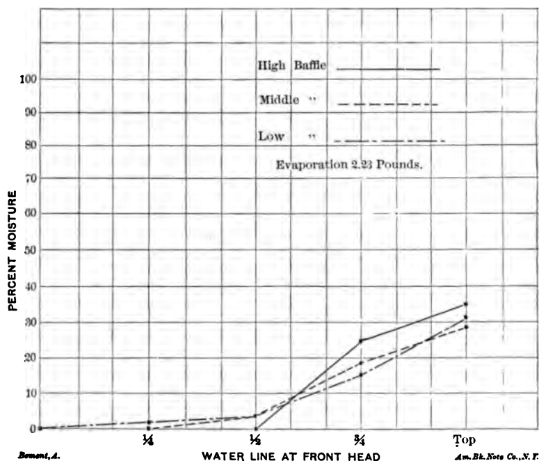
FIG. 98.—RESULTS OF TESTS OF BAFFLES.
