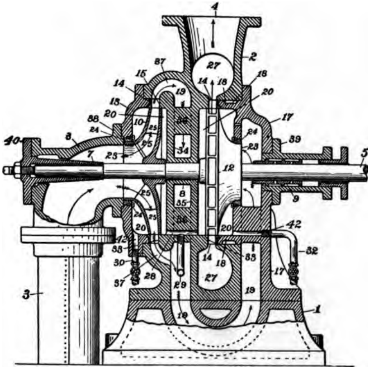
FIG. 274.—DETAILS OF THE J. RICHARDS COMPOUND ROTARY PUMP.
