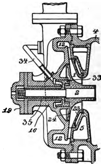
FIG. 267.—PARTIAL DETAIL OF THE A. C. E. RATEAU CENTRIFUGAL PUMP.
