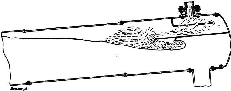
FIG. 103.—HIGH BAFFLE WITH MODERATELY HIGH WATER.
