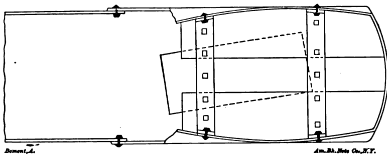
FIG. 113.—PLAN, PLATE COMPLETELY DETACHED.
