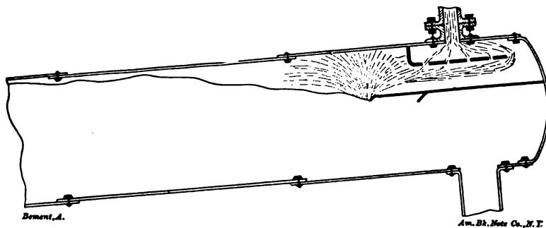
FIG. 102.—HIGH BAFFLE WITH HIGH WATER.
