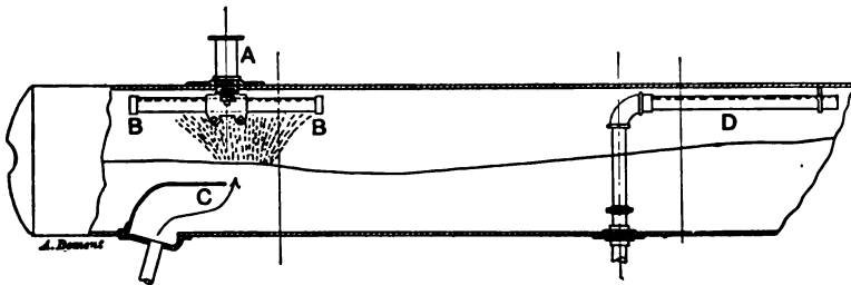
FIG. 226.—BOILER DRUM.
