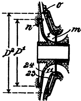
FIG. 270.—PARTIAL DETAIL OF THE A. C. E. RATEAU CENTRIFUGAL PUMP.
