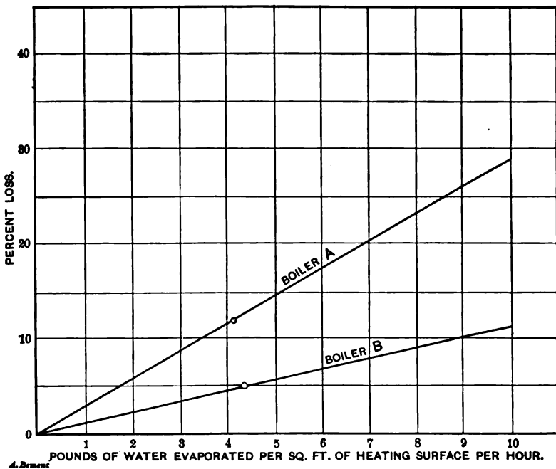
FIG. 234.—LOSS DUE TO INCREASING CAPACITY, MEASURED ABOVE STEAM TEMPERATURE.
