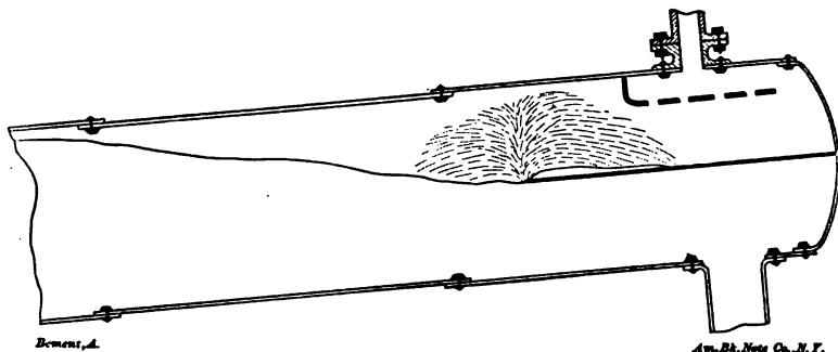
FIG. 101.—MIDDLE FORM OF BAFFLE.
