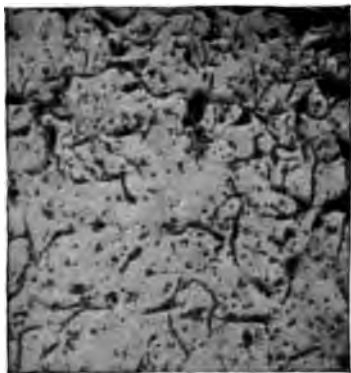
FIG. 166.—UNETCHED 100 DIAMETERS.
