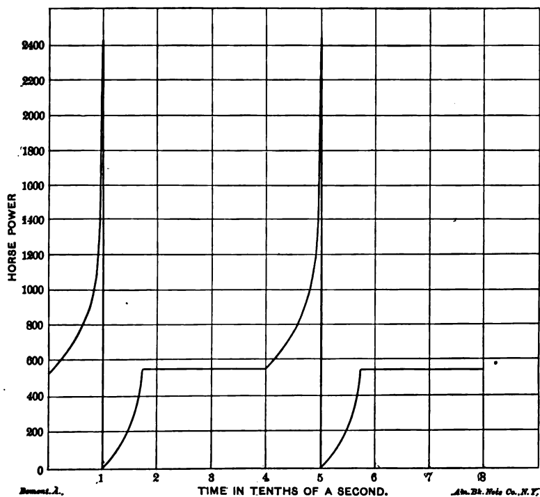
FIG. 116.—RATE OF EVAPORATION ONE BOILER, BOILERS OF GROUP No. 3 DURING ONE REVOLUTION OF ENGINES K AND L.
