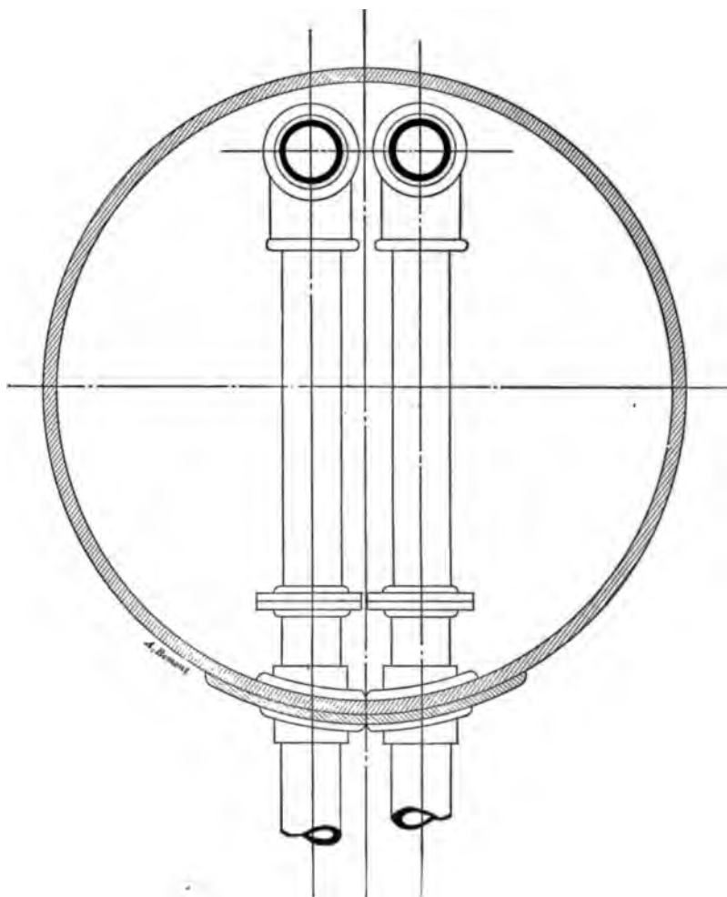
FIG. 228.—CROSS SECTION AT OUTLET TO SUPERHEATER.
