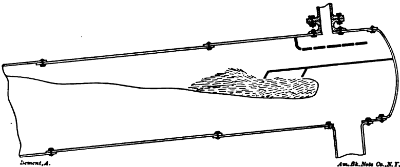
FIG. 104.—HIGH BAFFLE WITH NORMAL WATER LINE.
