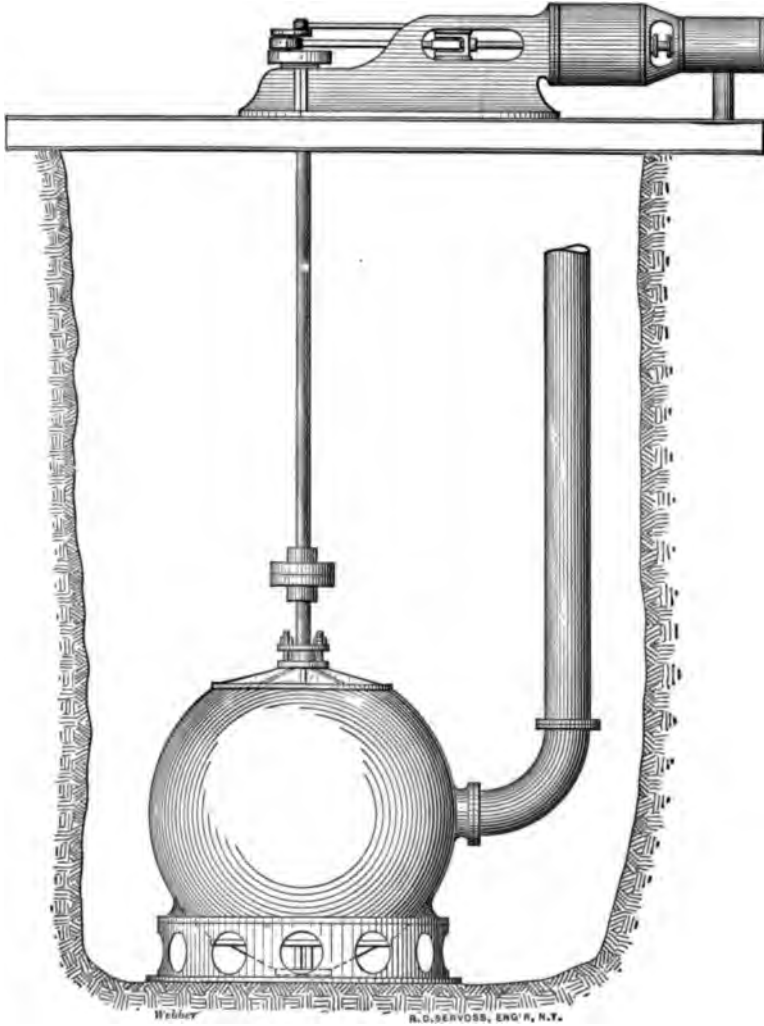
FIG. 281.—VERTICAL TURBINE PUMP.
