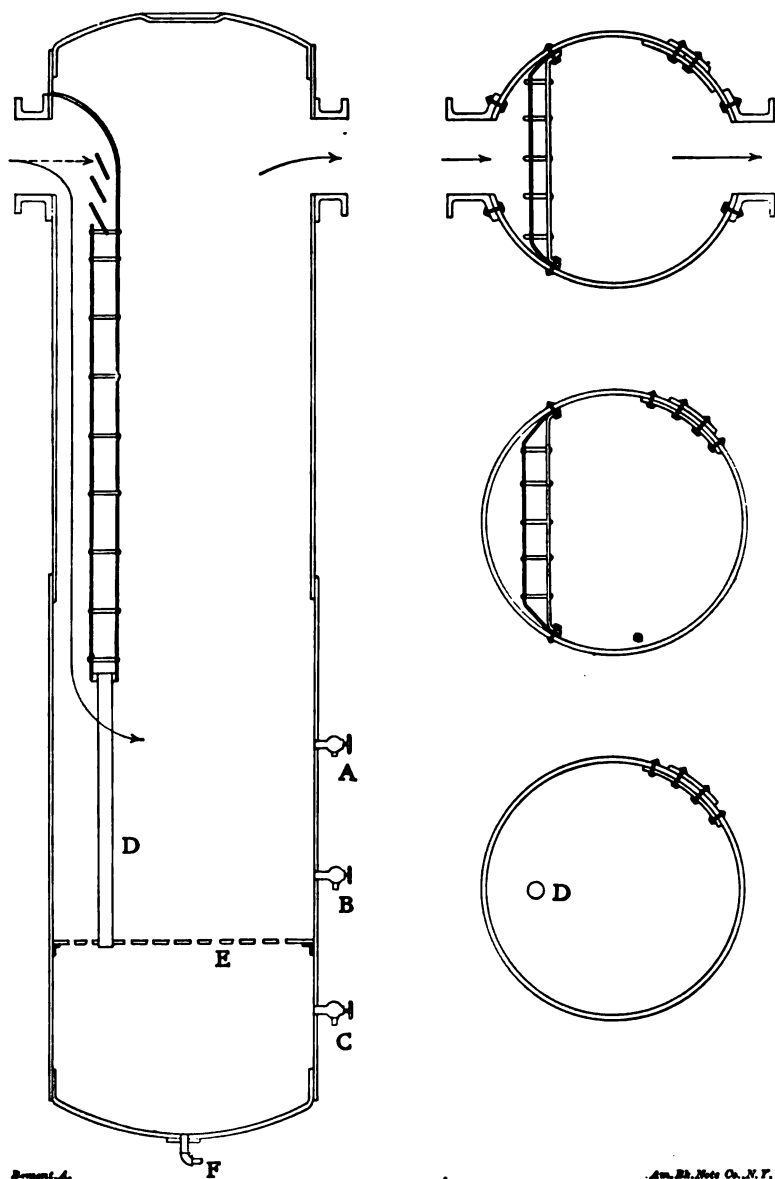
FIG. 117.—LARGE SEPARATORS. ENGINES K AND L.
