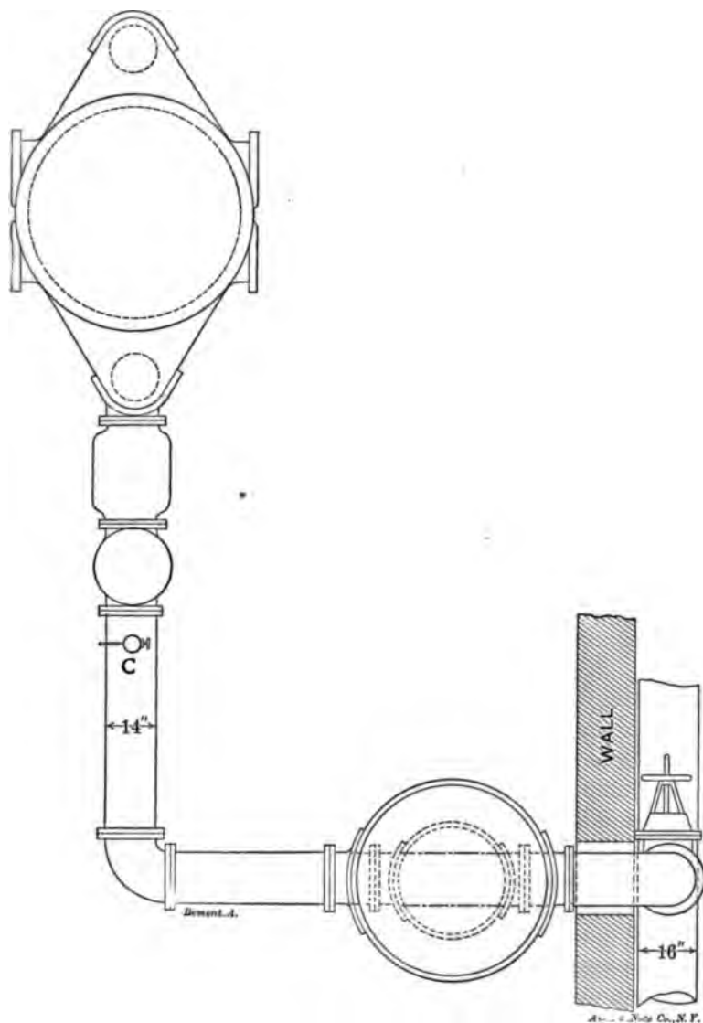
FIG. 110.—PLAN SHOWING DIFFERENT STEAM CONNECTIONS TO ENGINES K AND L.
