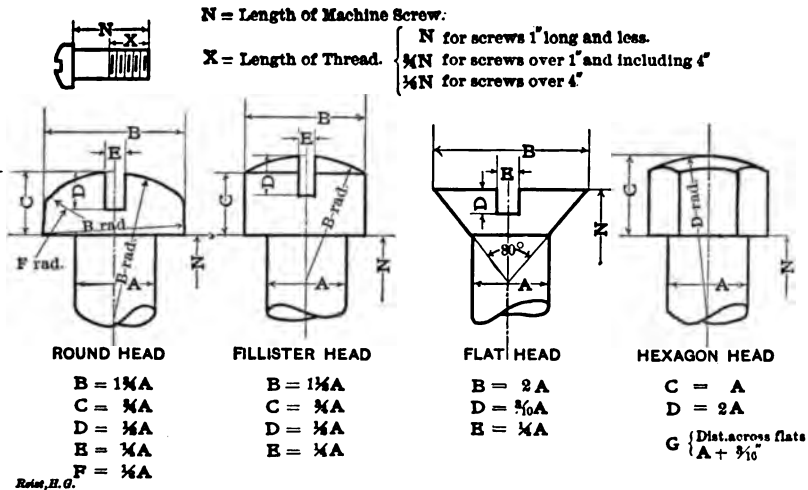
DIMENSIONS OF STANDARD MACHINE SCREWS.
