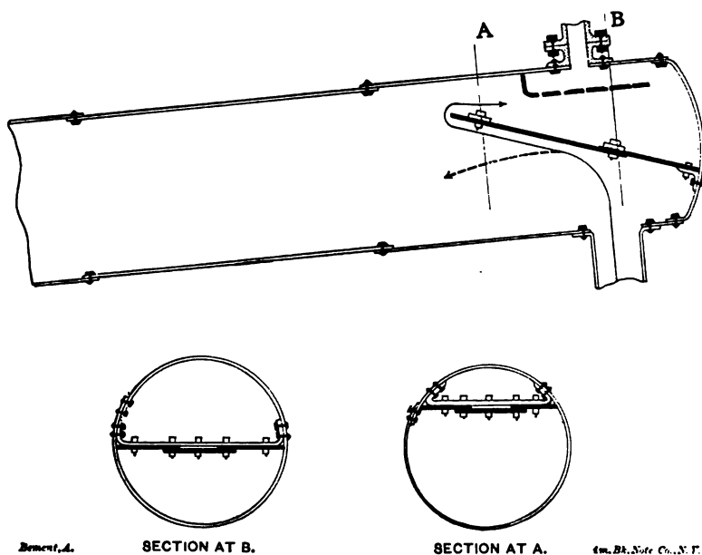
FIG. 94.—WATER BAFFLE IN HEINE BOILERS.
