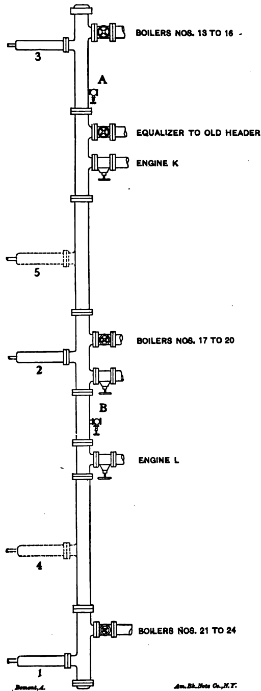
Fig. 108.—STEAM HEADER OF GROUP No. 3 SERVING ENGINES K AND L.
