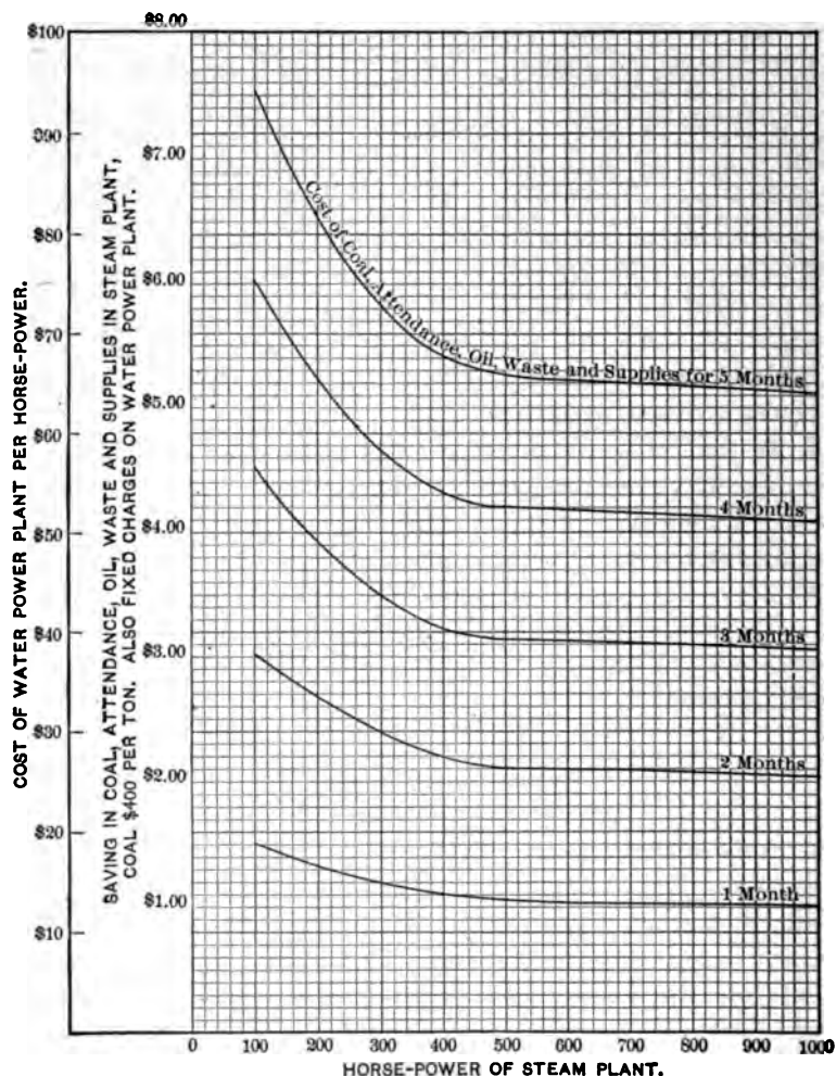
DIAGRAM SHOWING NUMBER OF MONTHS WHEN WATER SHOULD BE ALLOWED TO WASTE WITH DIFFERENT SIZES OF STEAM
