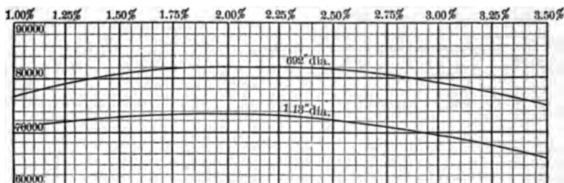
FIG. 145.—CHART OF CRUSHING STRENGTH SHOWING APPROXIMATE RELATION OF STRENGTH TO SIZE OF CASTING AND TO THE PERCENTAGE OF SILICON (Chart gives the strength per square inch.)
