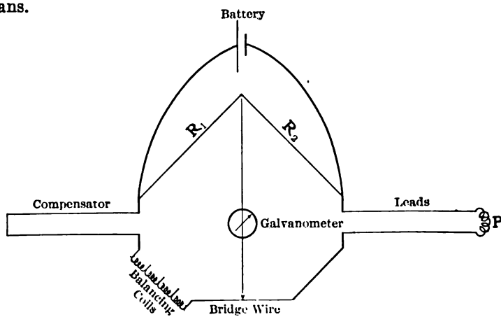
FIG. 205.—DIAGRAM OF PLATINUM THERMOMETER CONNECTIONS.
