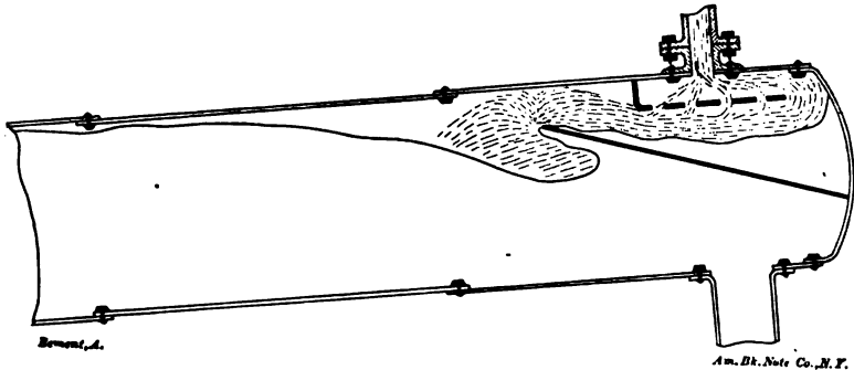
FIG. 99.—HEINE BAFFLE. HIGH WATER LINE.
