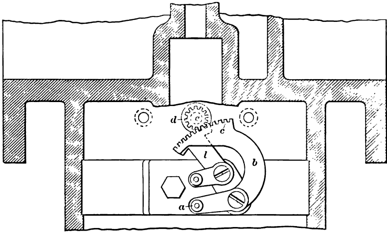
SECTION OF PLAN AND ELEVATION OF INDICATING LEVERS.
