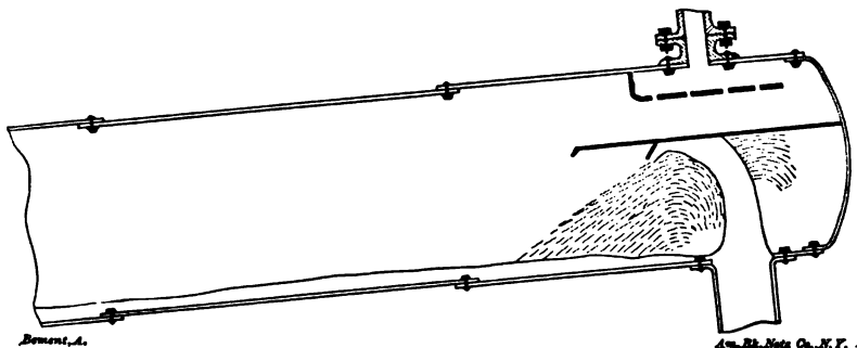
FIG. 105.—HIGH BAFFLE WITH LOW WATER.
