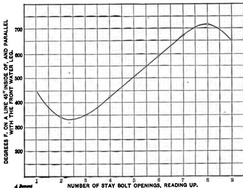
FIG. 233.—TEMPERATURE OF LINE Y OF FIG. 231.
