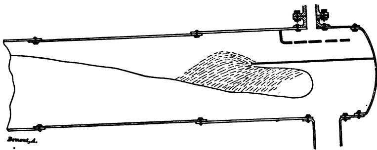
FIG. 106.—HIGH BAFFLE WITHOUT DEFLECTORS.
