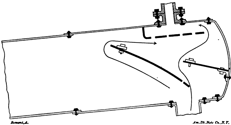
FIG. 114.—EXCEPTIONALLY DANGEROUS FAILURE IN BOILER No. 16.
