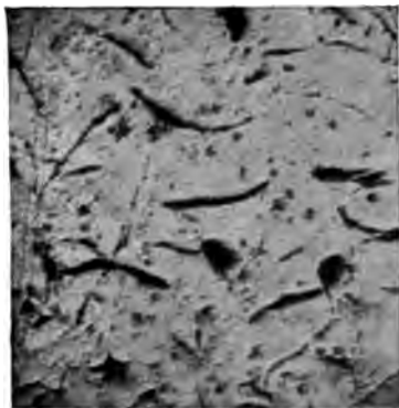
FIG. 172.—UNETCHED 100 DIAMETERS.
