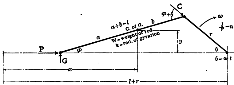
CONNECTING ROD DIAGRAM
